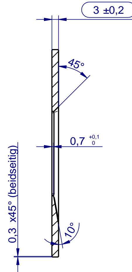
Detail B-B
